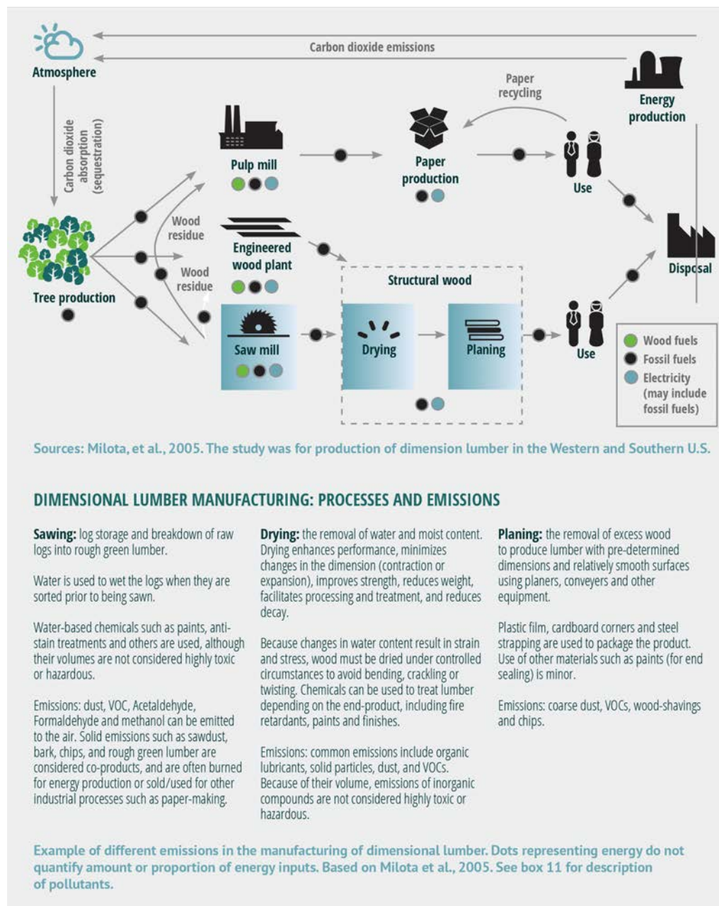
FIGURE 11. EXAMPLE OF EMISSIONS IN SOLID WOOD PRODUCTS
